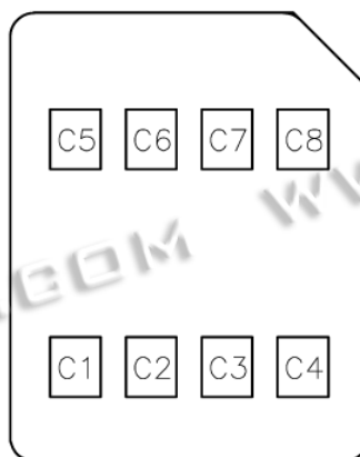
SIM CARD PAD LAYOUT
